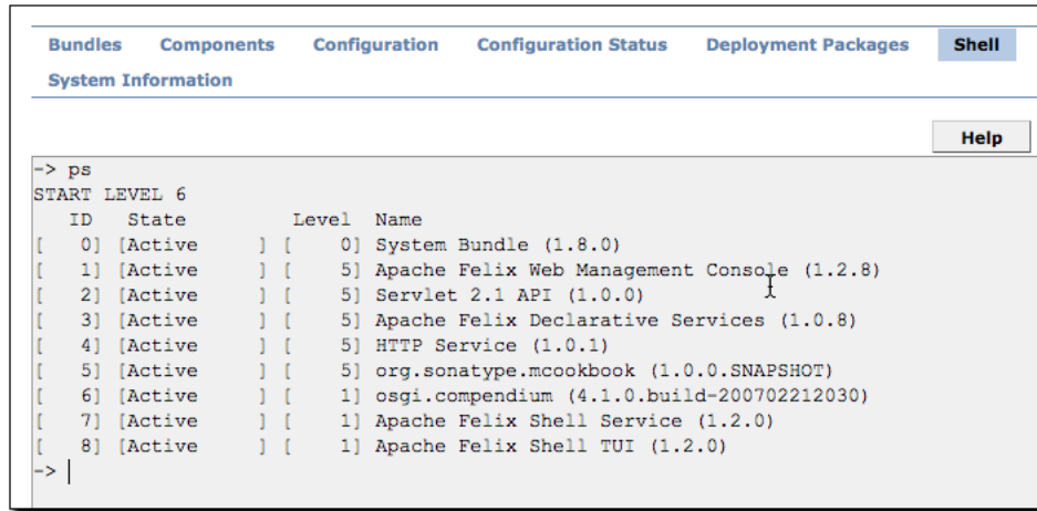
Figure 1.3. Running the Apache Felix Shell via the Administrative Web Console
